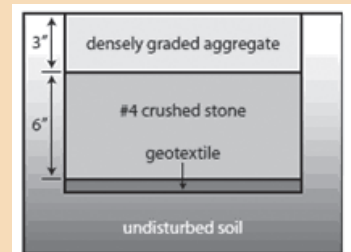
Figure 1. Construction details.
