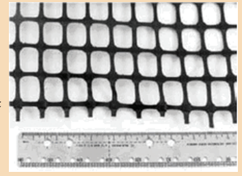
Figure 4. Geogrid for heavy-traffic areas.
