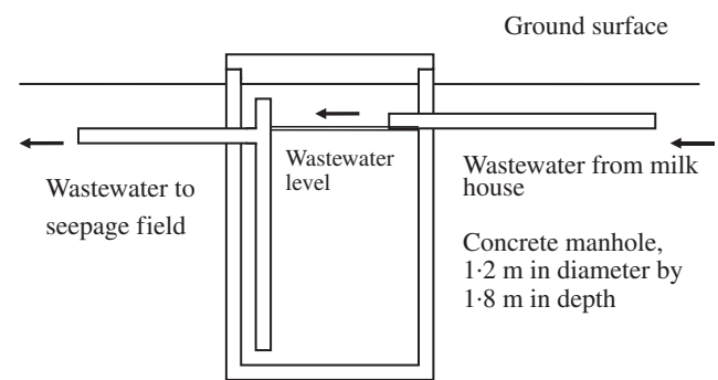
Fig. 1. Manhole used to collect milk house wastewaters intercepted before the septic tank system
